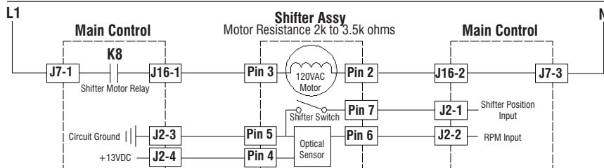
Figure 4 - Shifter Assembly Strip Circuit (Shifter Switch: Open = SPIN, Closed = AGITATE)
